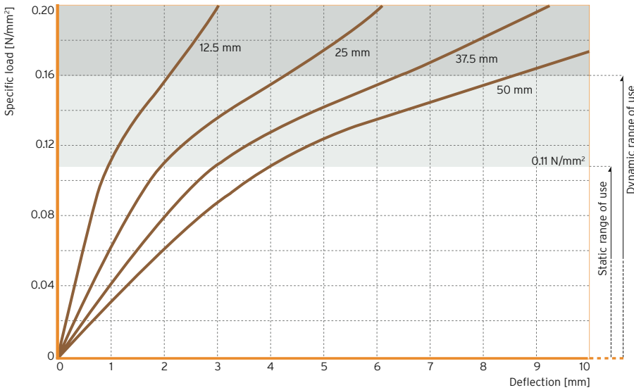
Figure 1: Quasistatic load deflection curve measured with a loading rate of 0.011 N/mm²/s
