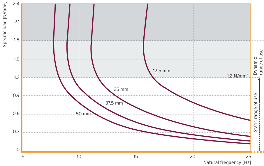
Figure 3: Natural frequency of a single-degree-of-freedom system (SDOF system) consisting of a fixed mass and an elastic bearing consisting of Sylomer® SR 1200 based on a stiff subgrade
