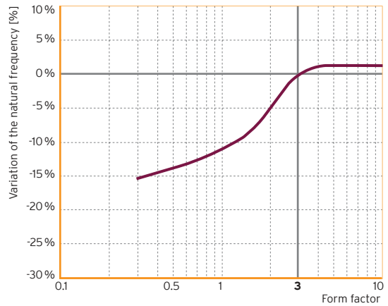
Figure 8: Natural frequency*
