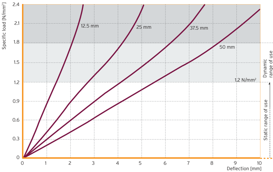
Figure 1: Quasistatic load deflection curve measured with a loading rate of 0.12 N/mm 2 /s
