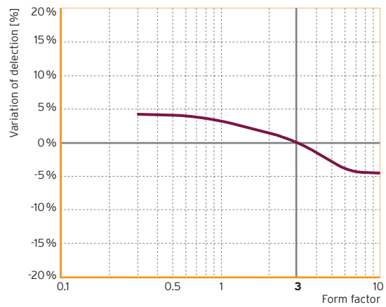
Figure 6: Deflection*
